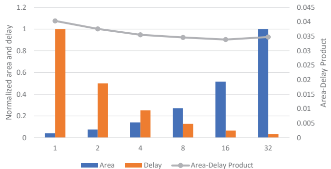
Fig. 7: Trade-off between area and number of cycles with varying values of the Parallelism knob (1024 input values, Accuracy=LUT, Storage=mem, Precision=float16)
